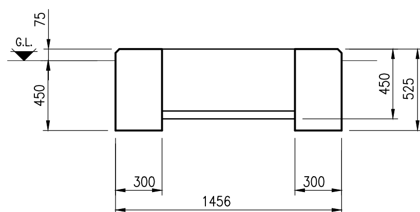
SECTION A-A CONCRETE GENERAL ARRANGEMENT
