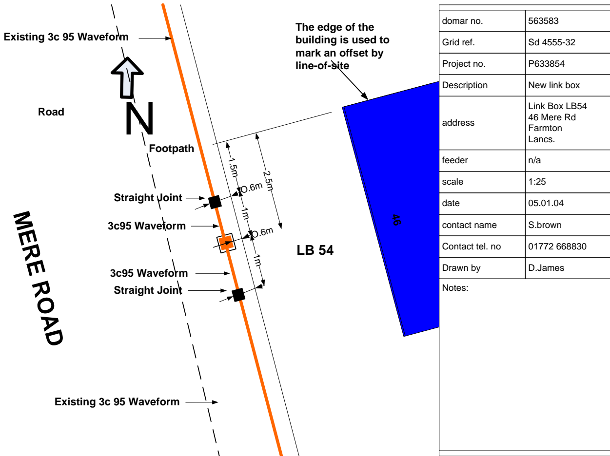
Figure 1 – Offset Method
