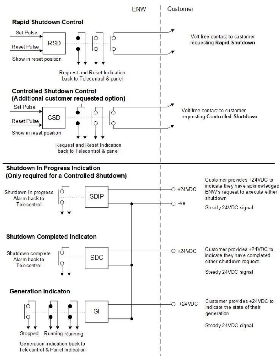
Generation Shutdown – Concept diagram
