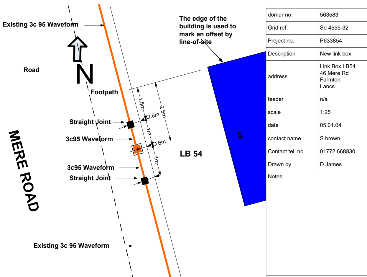
Figure 1 – Offset Method
