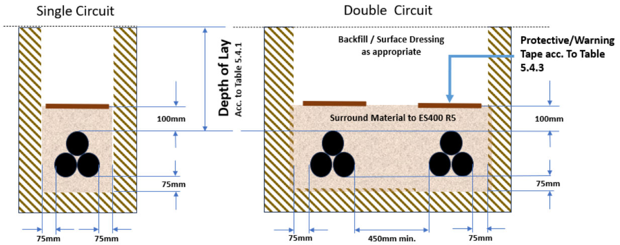
LAID DIRECT IN GROUND
