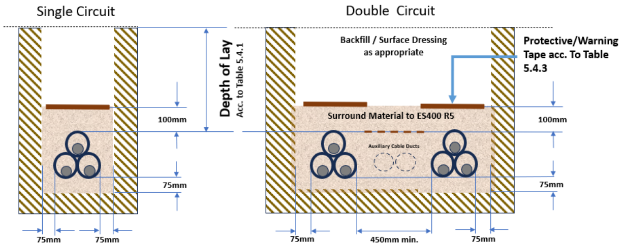
CABLES IN INDIVIDUAL DUCTS
